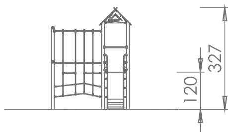
SCALE 1:200
